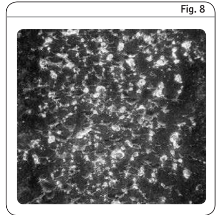
Microspalls and cracks on the raceway surface (high magnification)
