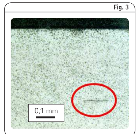
Crack development beneath the raceway surface (~ 0,3 mm)
