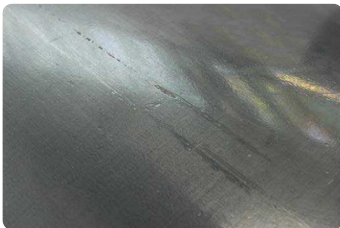
Tapered roller bearing outer ring
