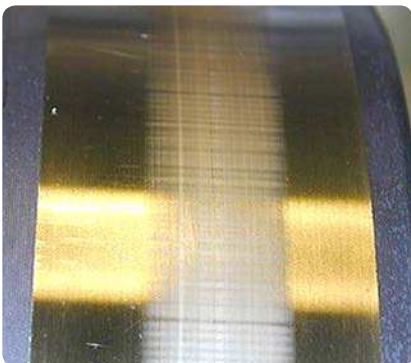
Washboarding on inner and outer rings and roller raceways
