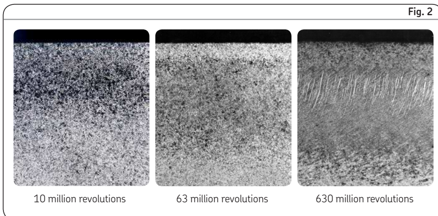
Changes in structure beneath the raceway surface over time (highly stressed, well lubricated small deep groove ball bearing)
