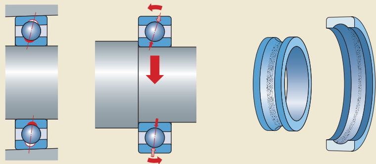
Load distribution
