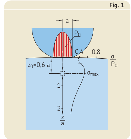
Compressive and shear stresses beneath the raceway
