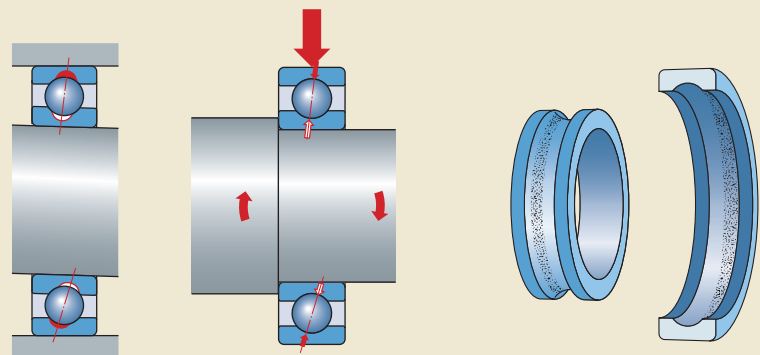
Load distribution
