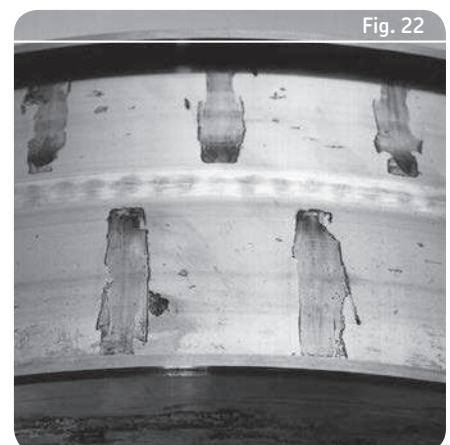
Initial patches of etching at rolling element pitch on the inner ring raceways of a spherical roller bearing
